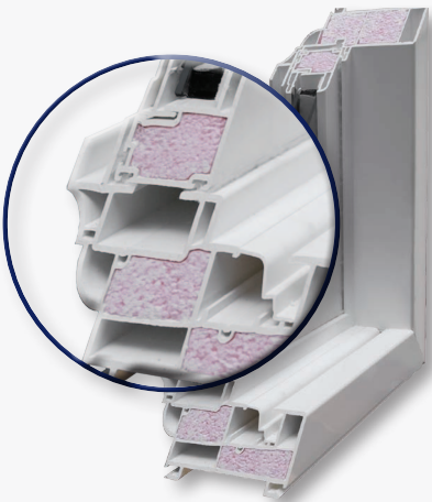
Foam Filled Extrusions to improve Energy Efficiency (Optional) — Shown DH800 —
